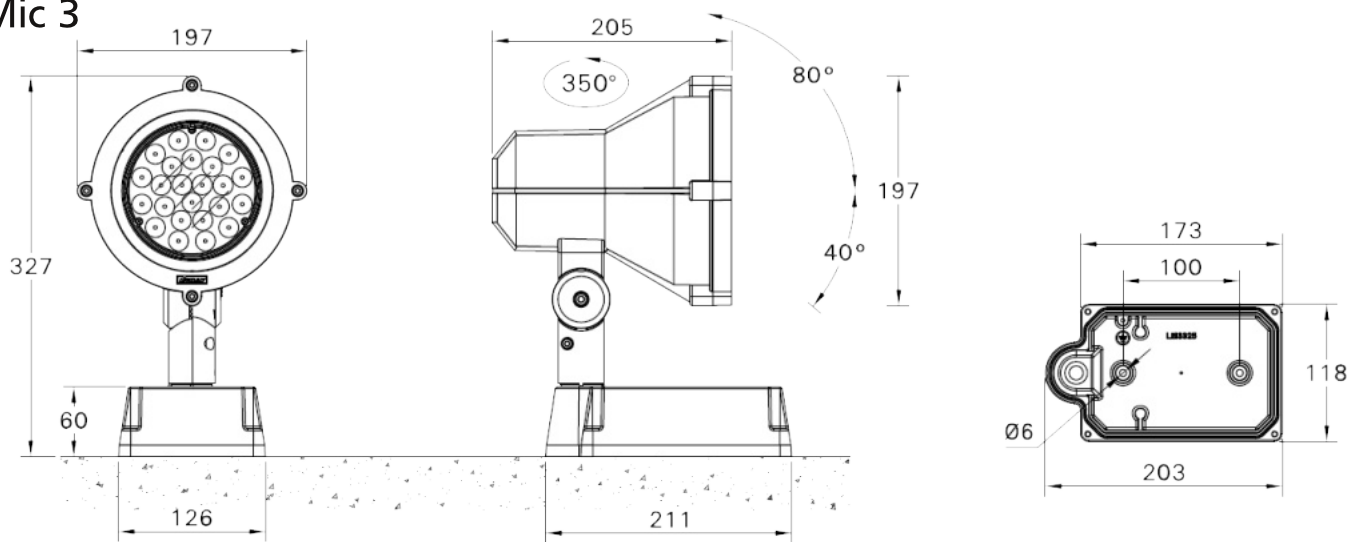
MOUNTING DETAIL
